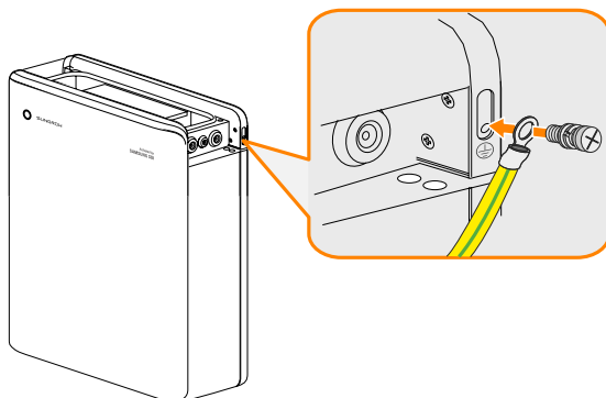
Figure 6-6 Connecting the protective earth cable
